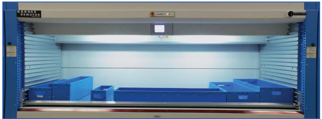
Interior of Remstar Vertical Shuttle. Shuttle trays are 3' x 10' Shuttles are 38' tall →
